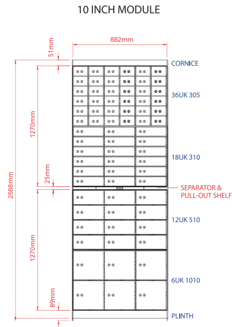
36UK 305 - 36 LOCKERS NETT WEIGHT : 183KG
